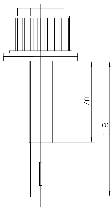
DM 20/120
