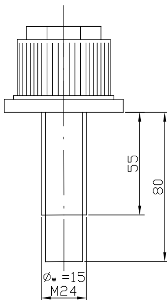
DM 24/80/55
