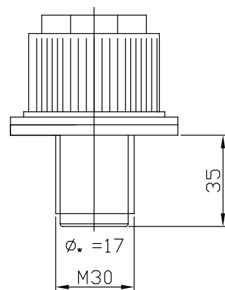
DM 30/30
