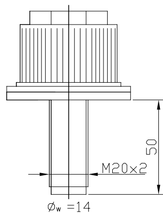
DM20x2/50
