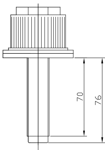
DM 20/70
