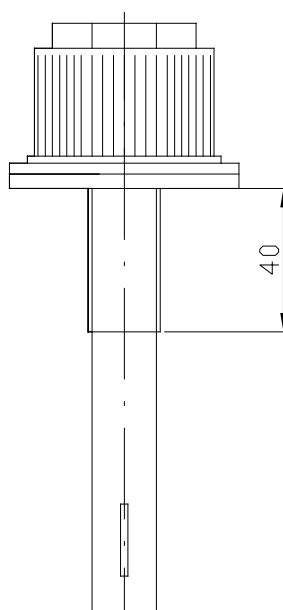
P1/120/40
