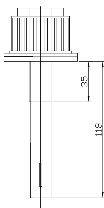
DM 20/120/35
