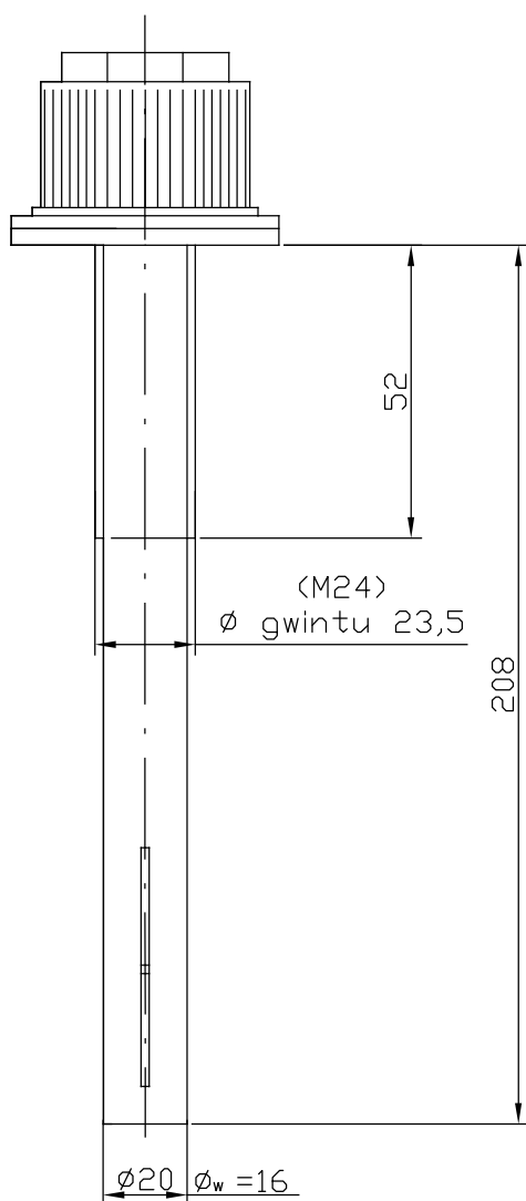
DM 24/S
