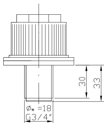
DG 3/4"/30
