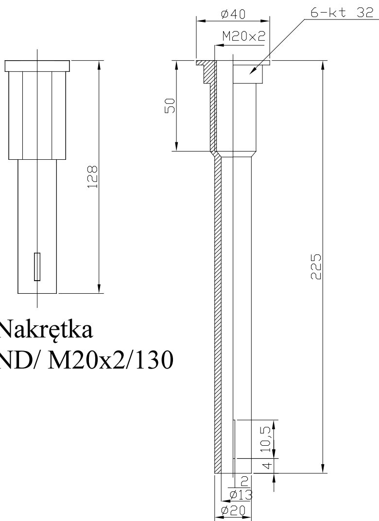
ND/M20x2/225
