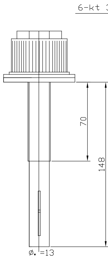
DM 20/150
