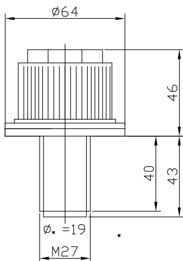
DM 27/40
